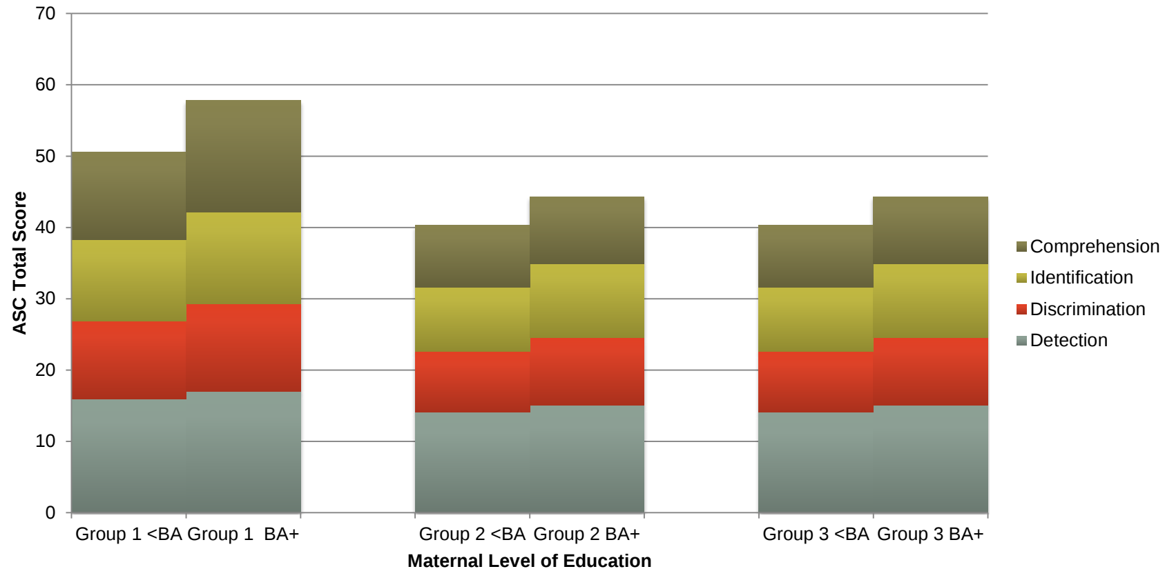
Comparison of Subscale Scores Based on MLE and HL
